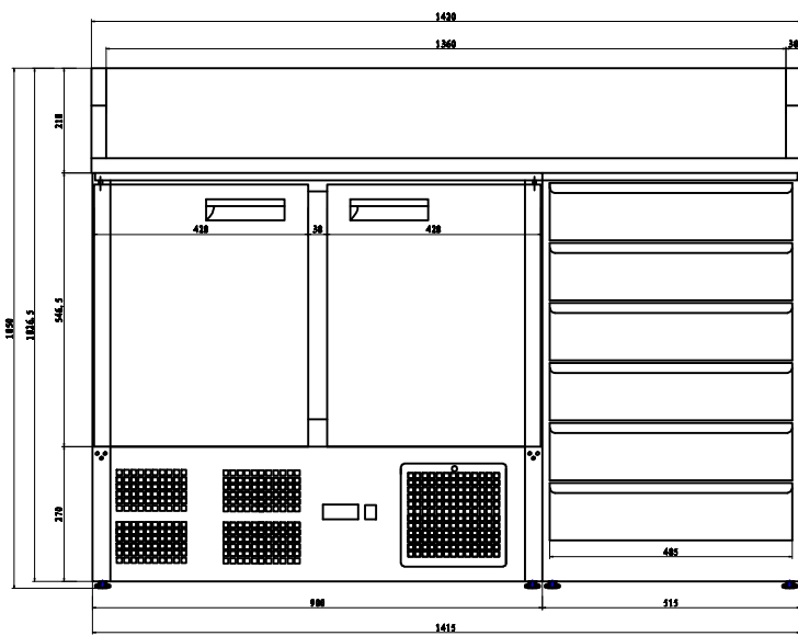
OUTSIDE DRAWING OF G-PZ9001
