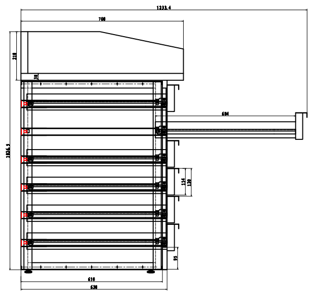
OUTSIDE DRAWING OF G-PZ9001
